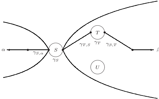
Figure 4. If \gamma_{T,S} avoids U , then \alpha, \beta are \mathcal{G}_U -connected.
