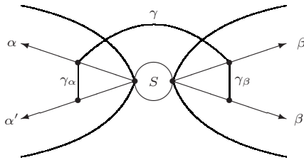
Figure 2. If \alpha, \beta are \mathcal{G}_S -connected, then so too are \alpha', \beta' .
